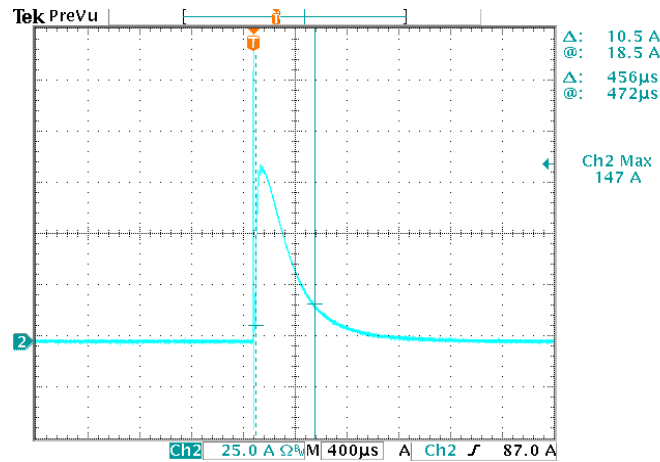
EUK-150S105DT(TT)( I_o=700mA )
