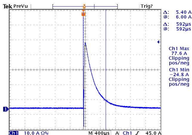
EUK-240S105DT(TT)( I_o=700\text{mA} )
