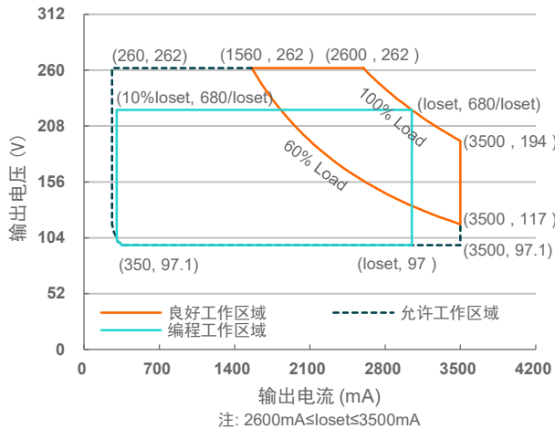
EUM-680S350BG
