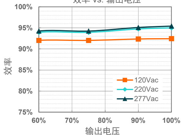
EUM-680S350BG( I_o=3500mA )
