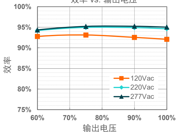
EUM-680S350BG( I_o=2600mA )
