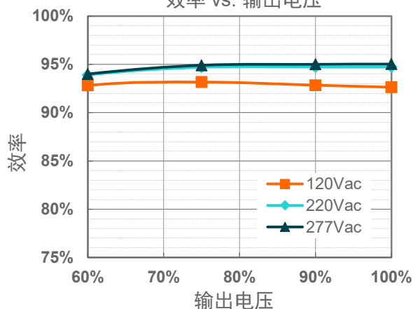
EUM-680S15ABG( I_o=12600mA )
