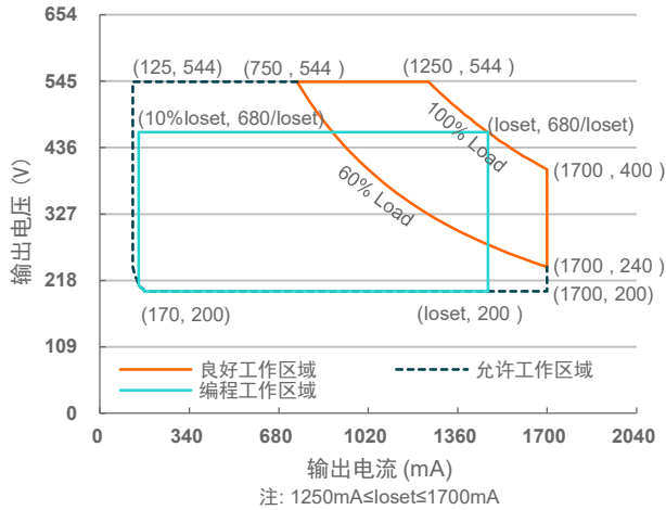
EUM-680S170BG
