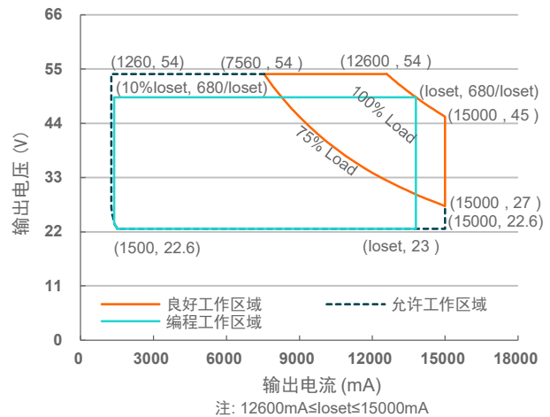
EUM-680S15ABG
