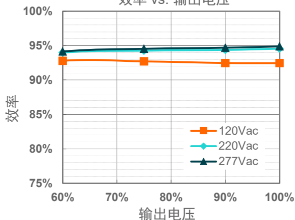
EUM-680S350BG( I_o=2600mA )
