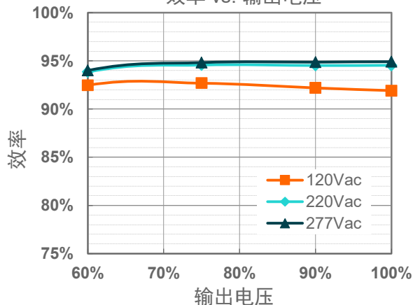
EUM-680S840BG( I_o=6300mA )
