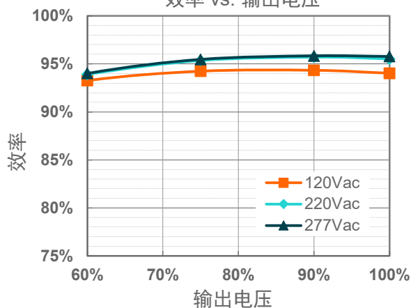
EUM-680S15ABG( I_o=12600mA )
