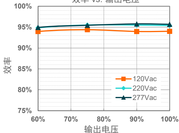
EUM-680S240BG( I_o=1800mA )
