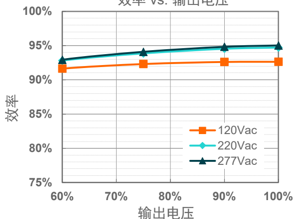
EUM-680S15ABG( I_o=15000mA )
