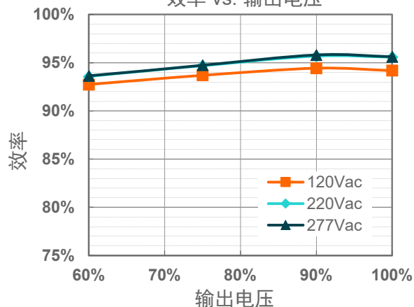
EUM-680S240BG( I_o=2400mA )
