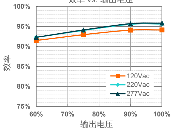
EUM-680S15ABG( I_o=15000mA )
