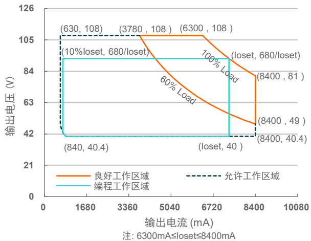
EUM-680S840BG
