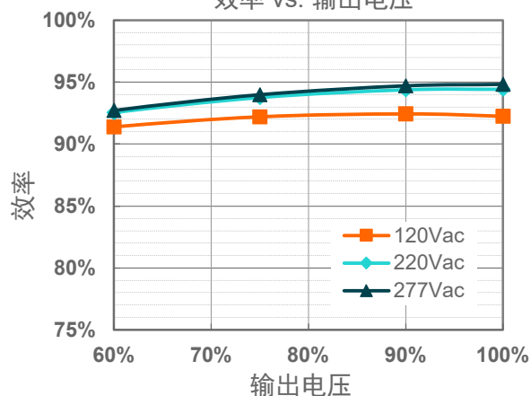
EUM-680S350BG( I_o=3500mA )
