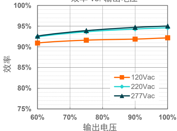
EUM-680S840BG( I_o=8400mA )
