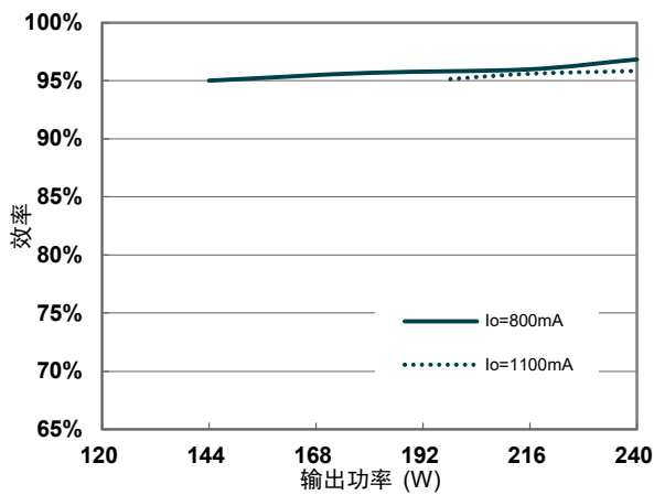
效率@230Vac
