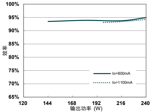
效率@230Vac
