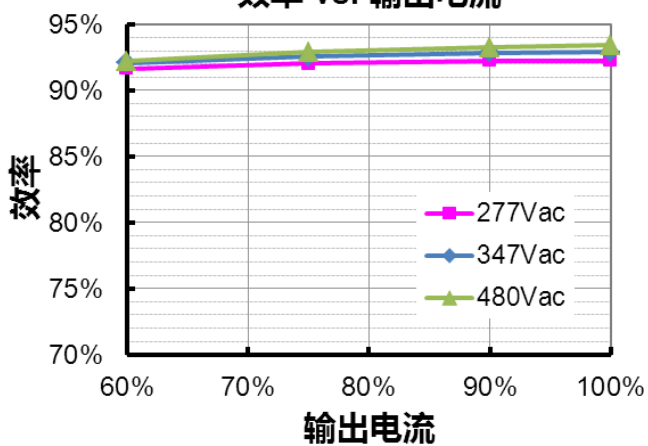
ESV-320S054SV 效率 vs. 输出电流
