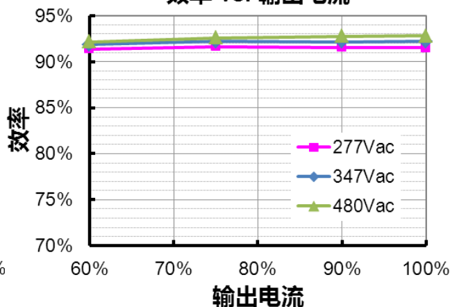
ESV-320S054SV 效率 vs. 输出电流
