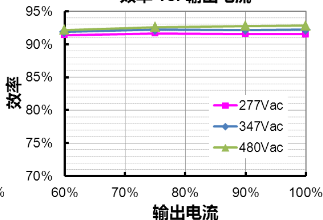
ESV-320S054ST 效率 vs. 输出电流
